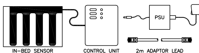
E50314 BED EPILEPSY KIT
